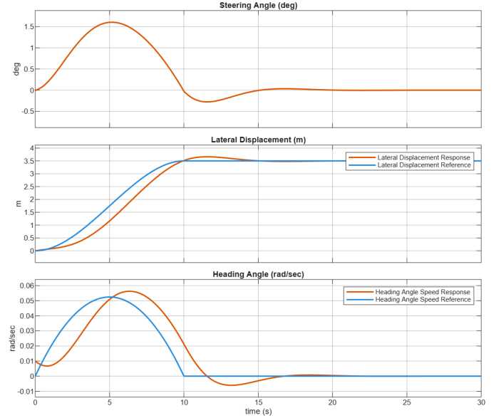
Fig. 3. Lateral displacement tracking performance for the lane-change maneuver using the ADRC-based controller. The ADRC achieves accurate tracking with zero steady-state error despite model uncertainties and external disturbances.
